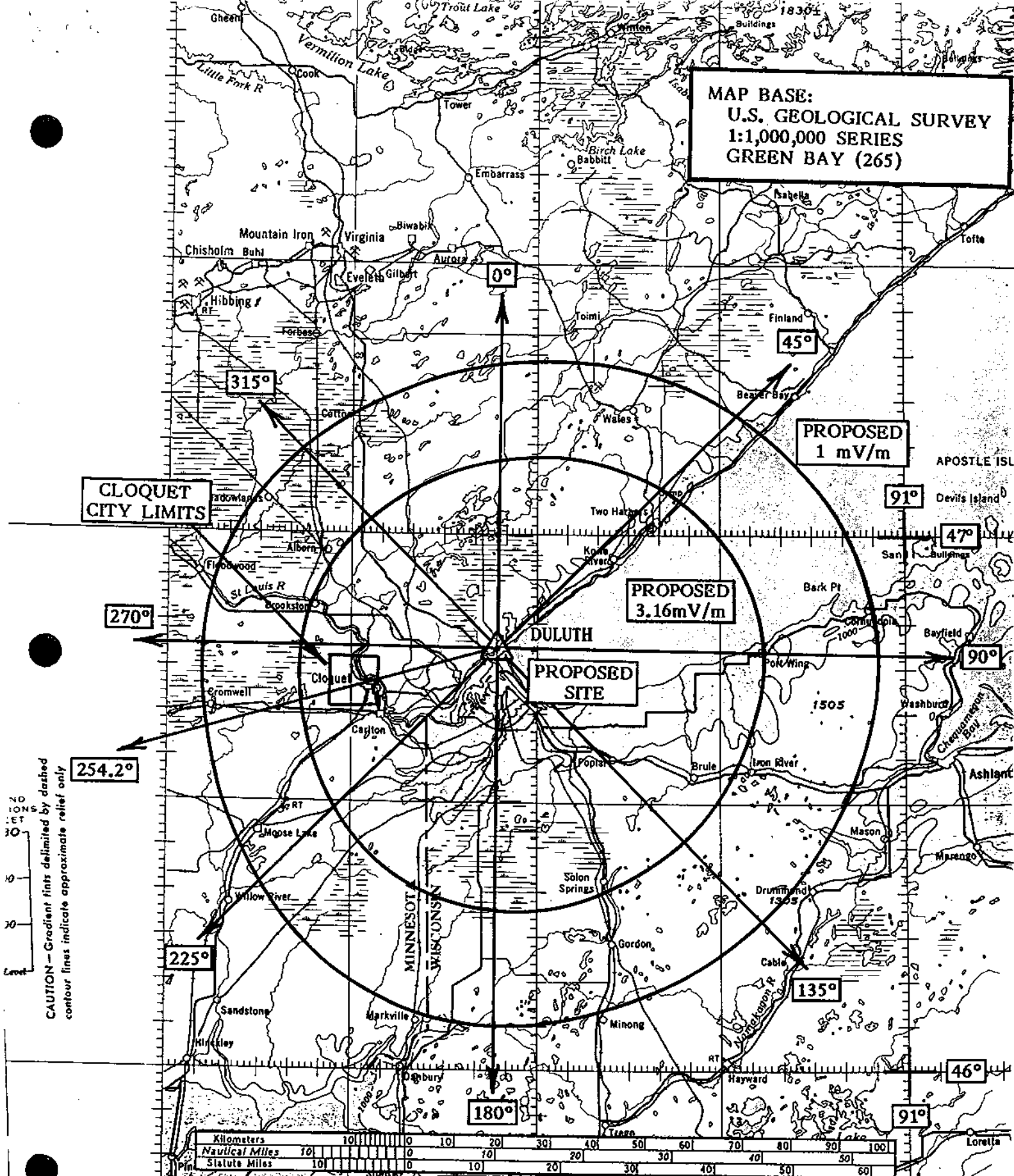
FIG. 4.9 WSCN PREDICTED PROPOSED SERVICE CONTOURS Minnesota Public Radio Cloquet, MN
